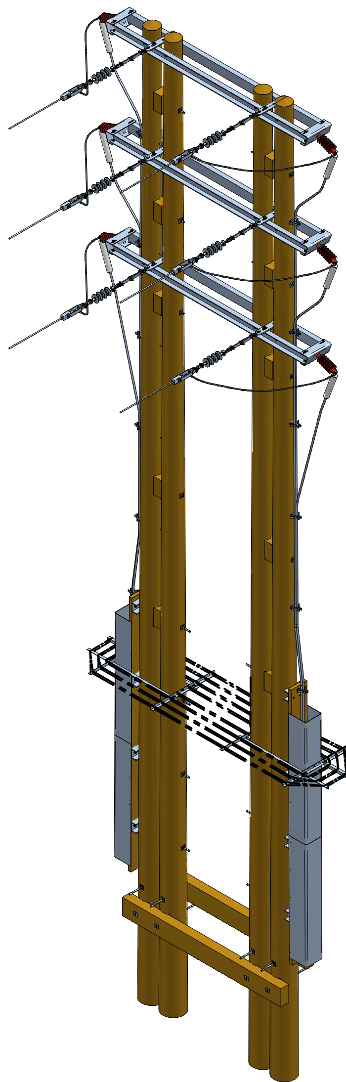
ISOMETRIC VIEW (ILLUSTRATIVE ONLY)
