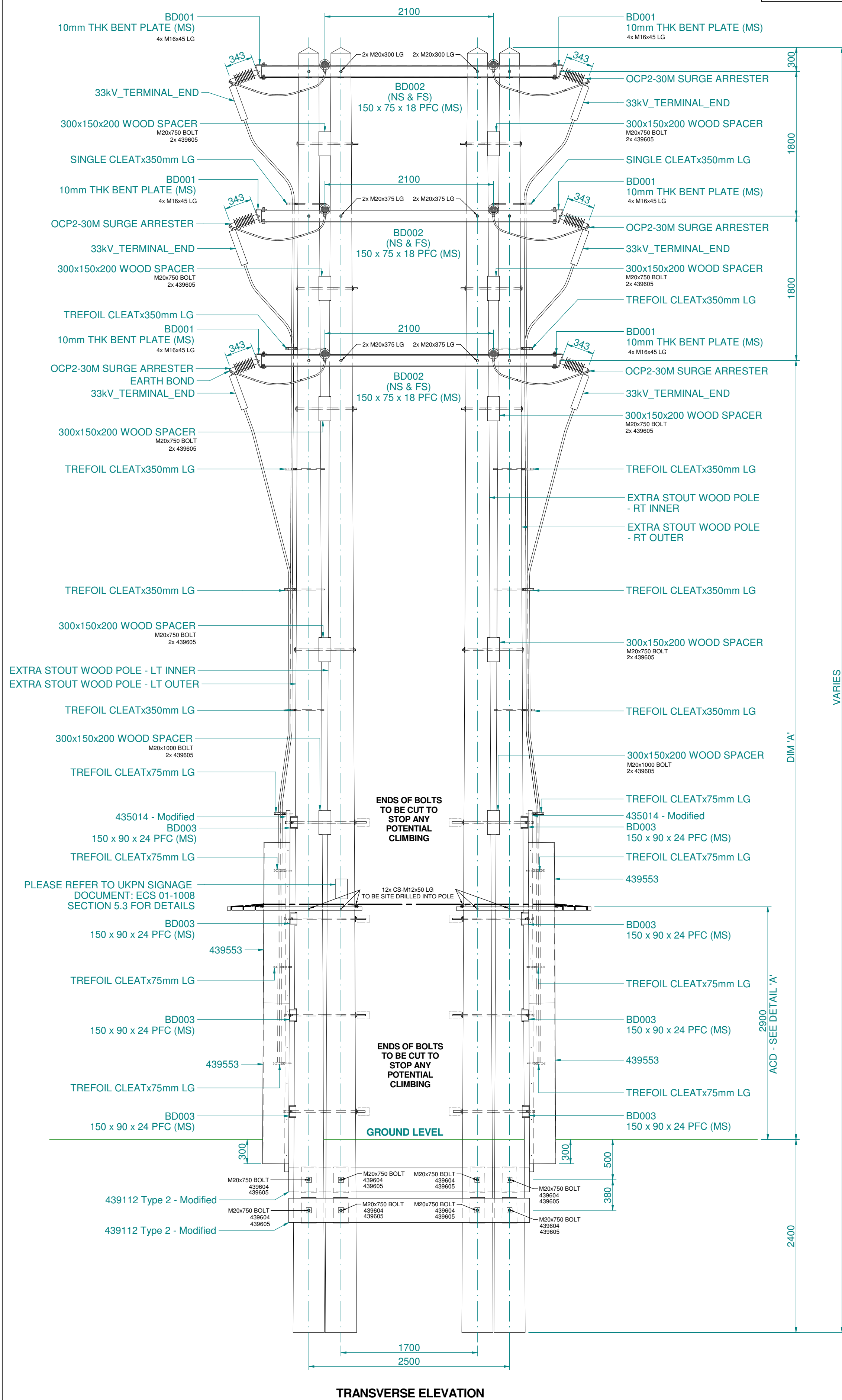
TRANSVERSE ELEVATION
