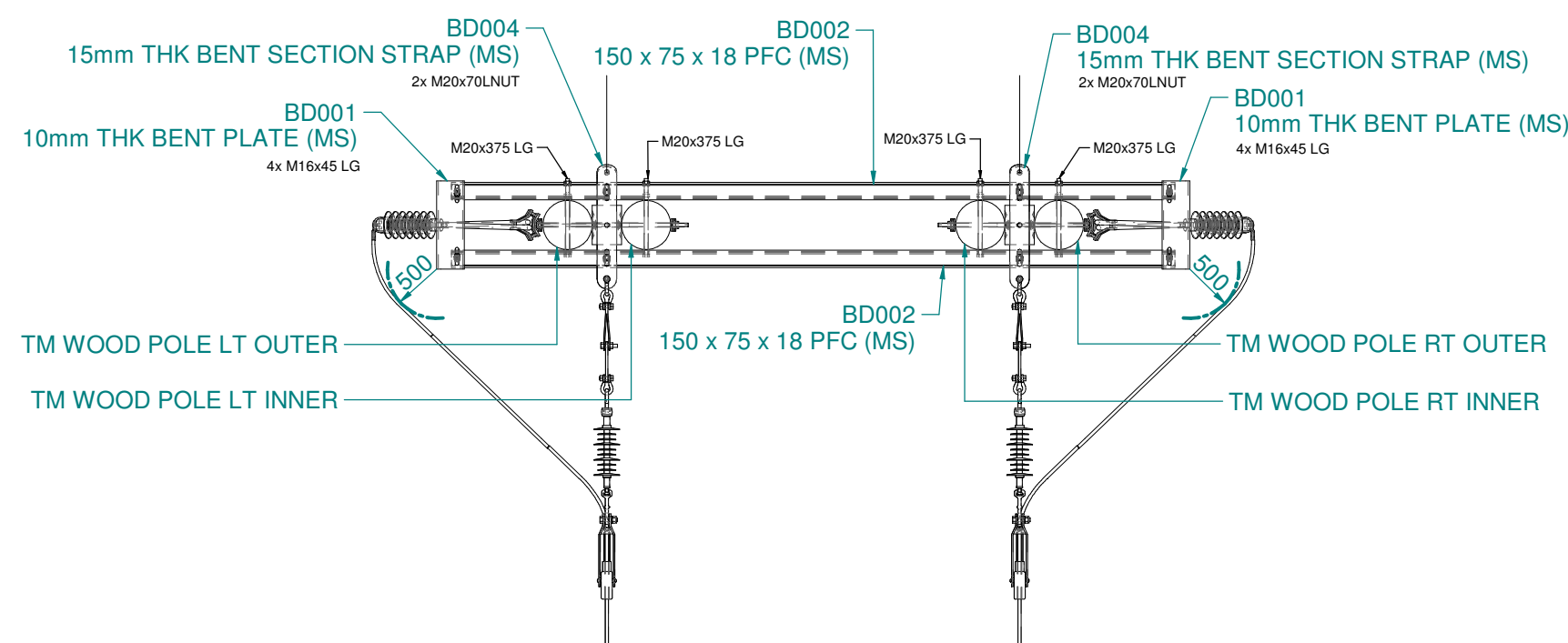
TYPICAL PLAN VIEW OF CROSSARM
