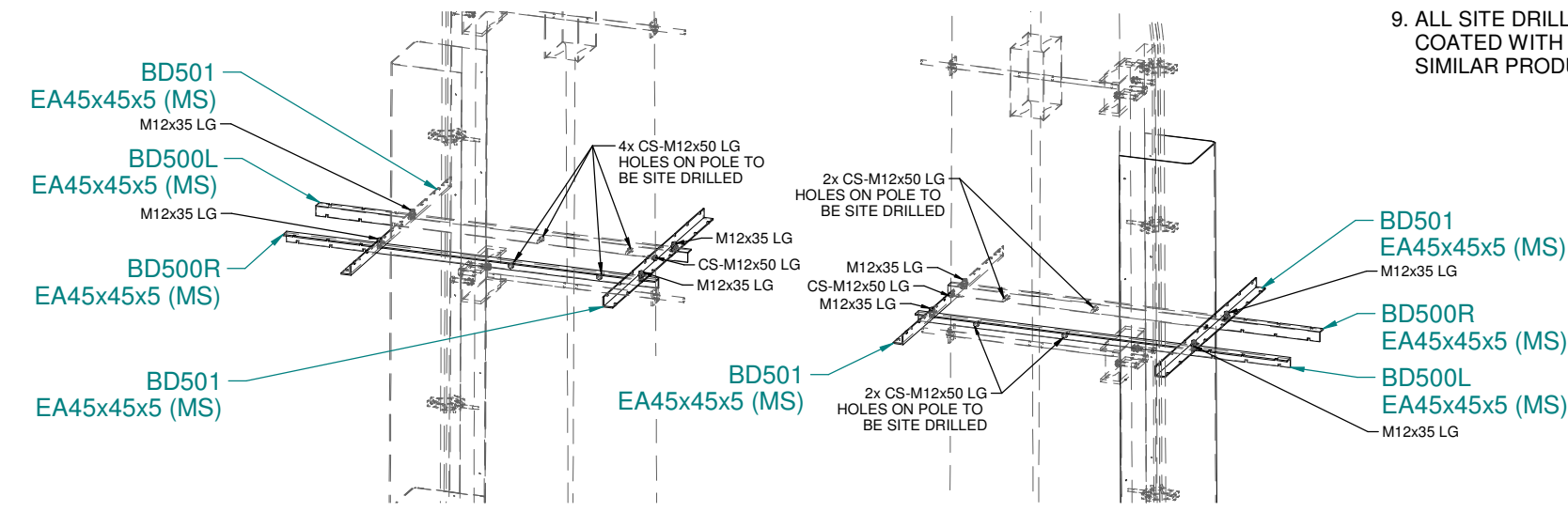
DETAIL 'A' VIEW OF ACD
